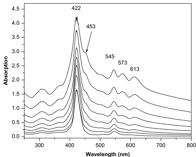
Figure 2. Dilution of a concentrated dispersion of 4h-Zn in dry dichloromethane. The concentrations from the top trace to the bottom trace were (mM): 1.5, 1.0, 0.6, 0.48, 0.36, 0.3, 0.2, 0.15. The strongly light scattering suspension of the more concentrated dispersion lead to a baseline shift, which was not corrected in the spectra (raw data are presented). The topmost trace slightly saturates the detector at the Soret band (422 nm) of the monomeric form.
