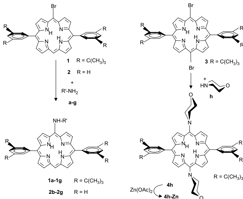
Scheme 1. See Table 1 for reaction conditions and yields.
